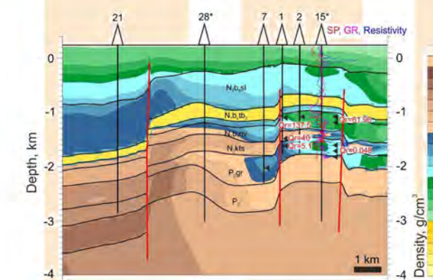
Figure 5. Conformal density slice within Paleogene
