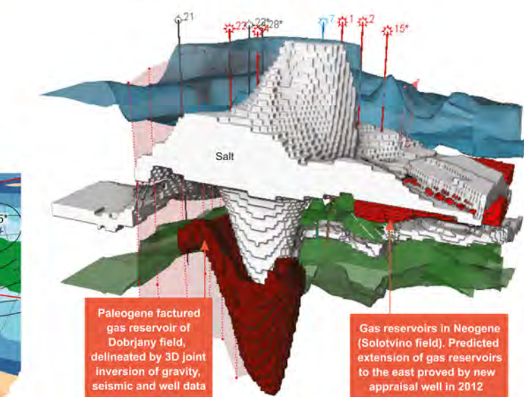
Figure 8. Neogene salt (in gray), Neogene and Paleogene gas pools (in red and dark red respectively), extracted in form of bodies from the inverted 3D density model
