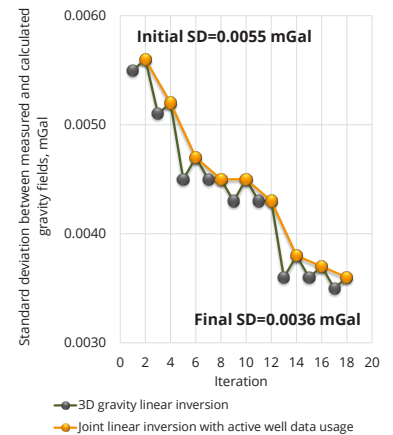
Figure 5. Iterational refining of the 3D density model during 3D gravity-inversion
